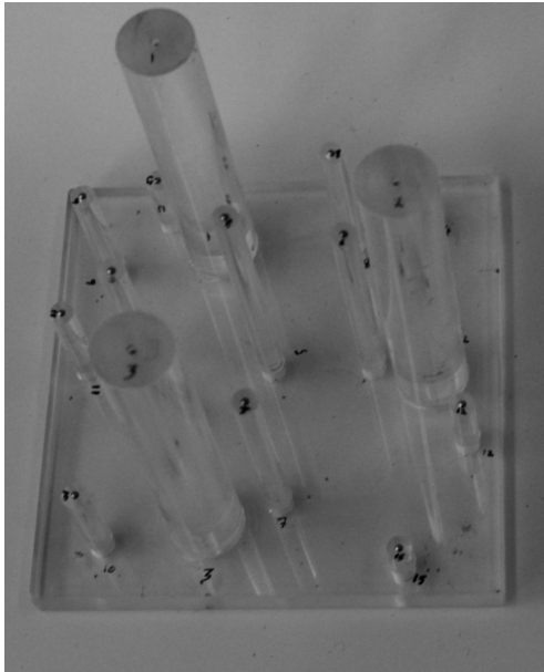
Figure 3.5: Spatial accuracy test phantom.
