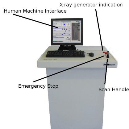
Figure 2.4: Control Computer on the Lodox Statscan.
