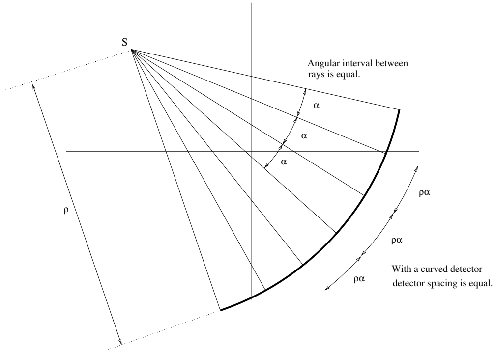
Figure 2.13: Equiangular fan beam.
