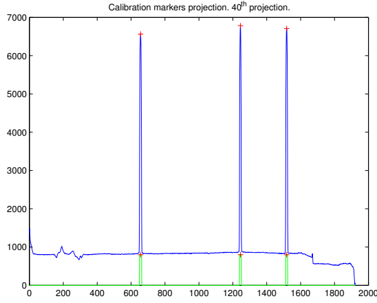
Figure 3.22: Plot of projection of pins, threshold output and pin medians.
