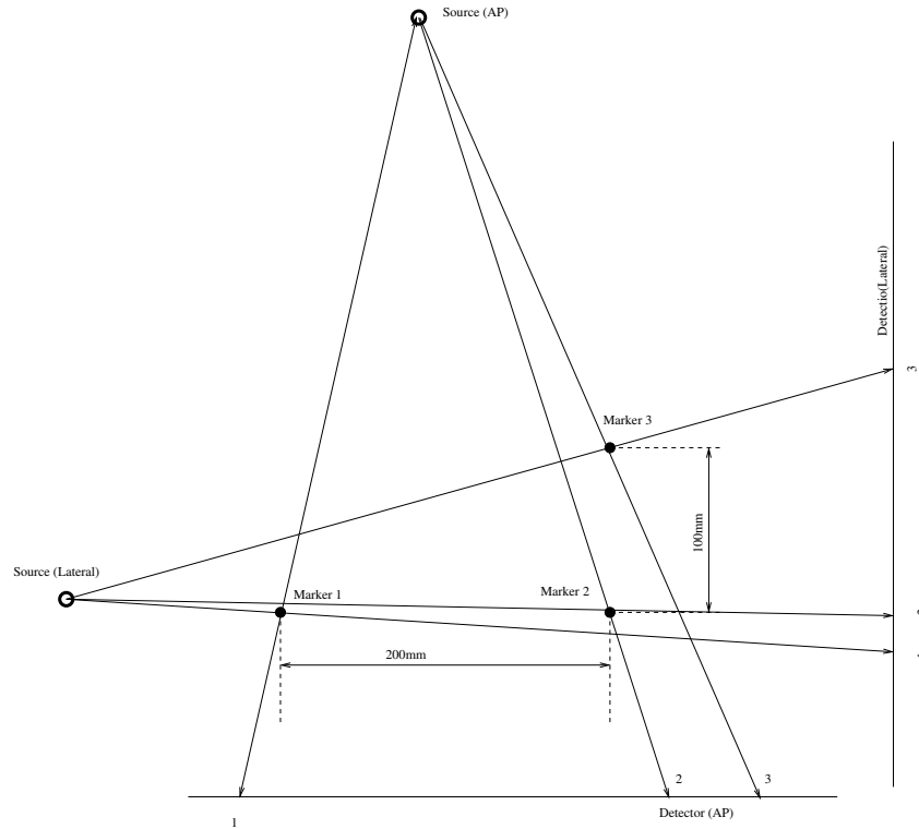
Figure 3.21: Pin locations and simulated projection.
