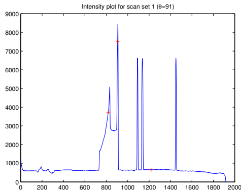
Figure 4.8: Intensity plot for scan set 1 projection 91 ( \theta_{c-arm} = 90^\circ ).
